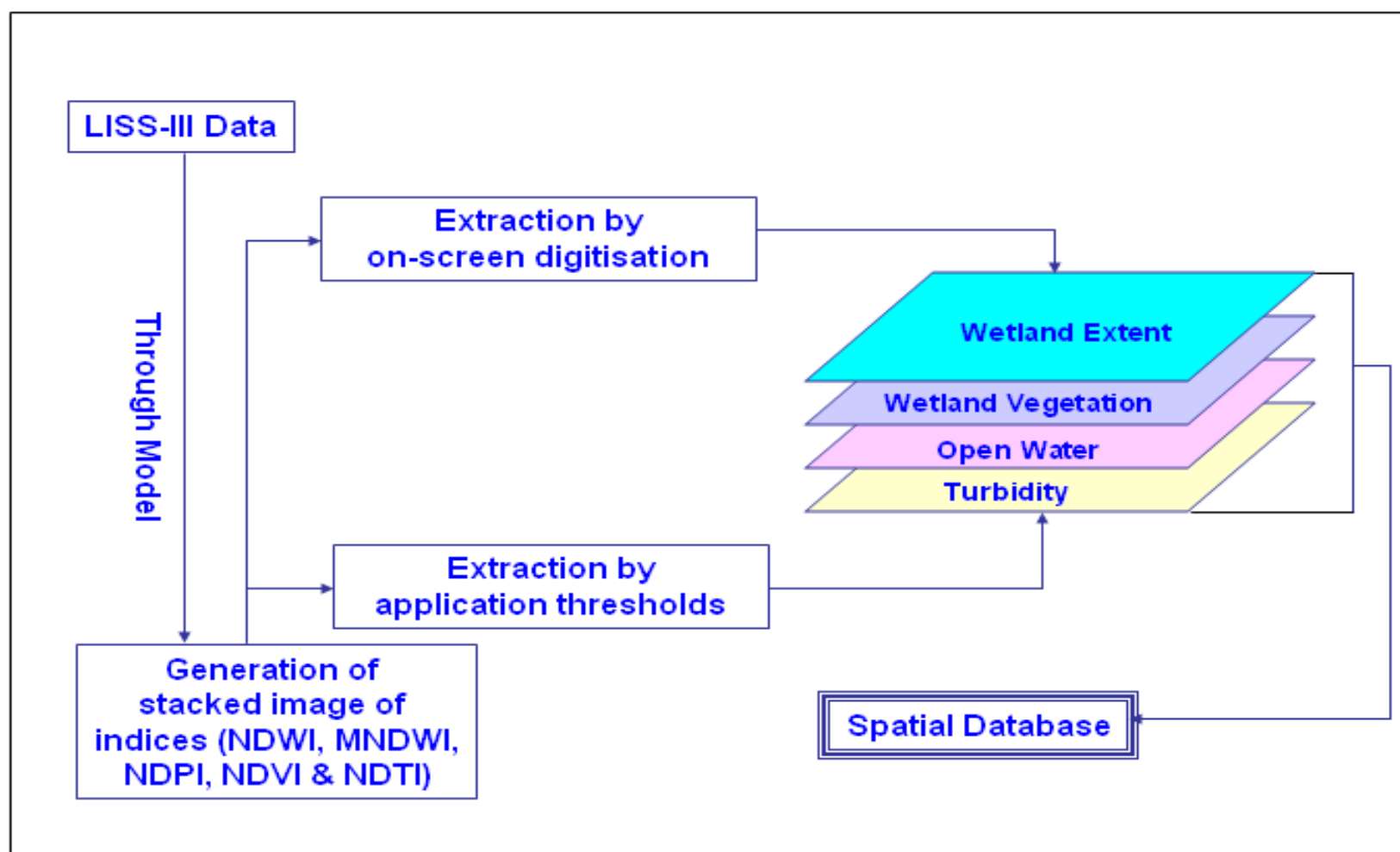
Figure 9: Steps in the extraction of wetland components
