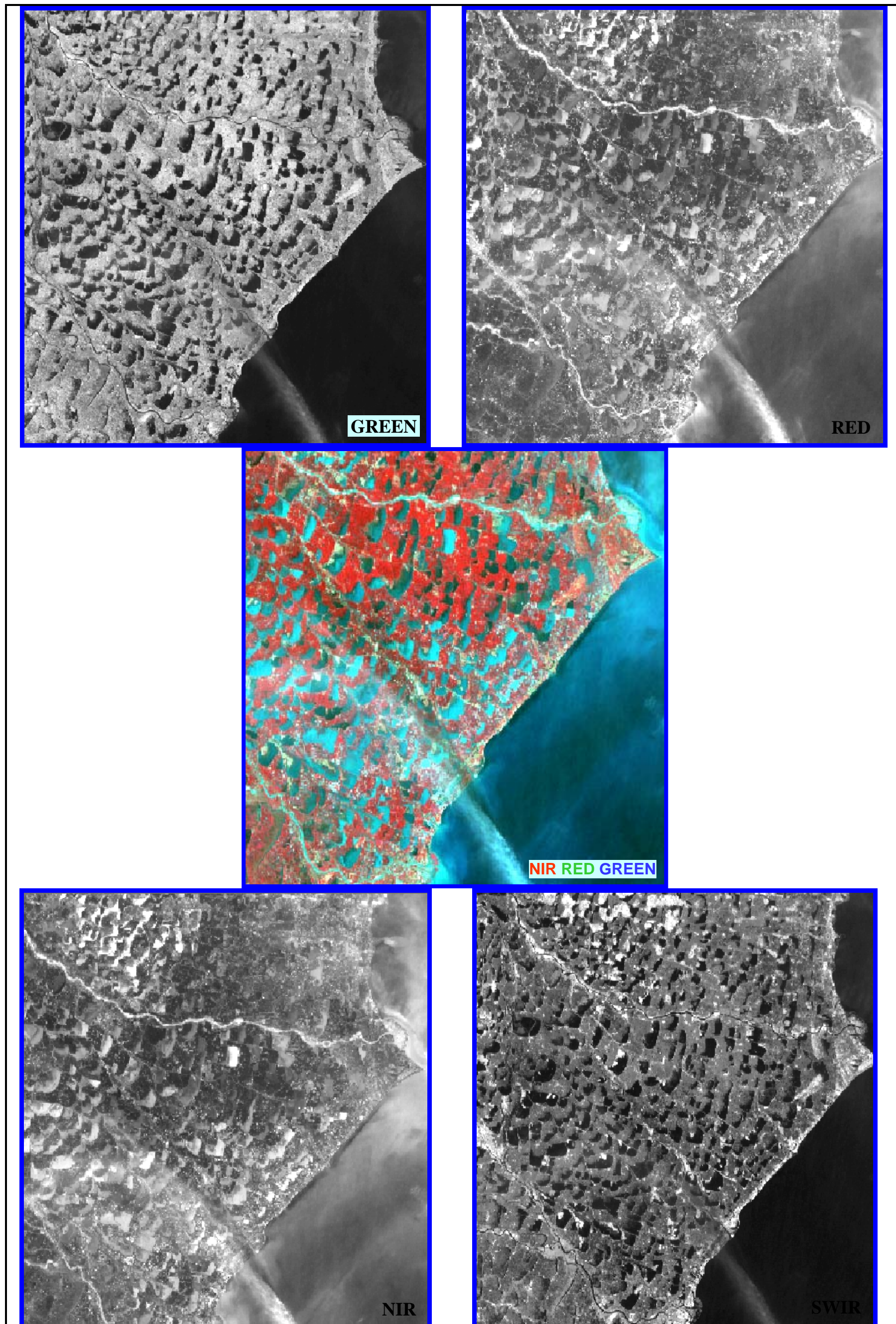
Figure 2: Various wetland features as they appear in four spectral bands and in a typical three-band FCC (part of Tamilnadu)
